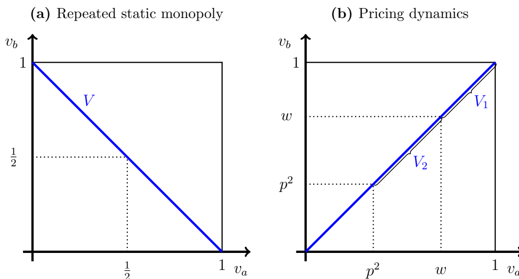
Figure 5: Two examples with linear support
